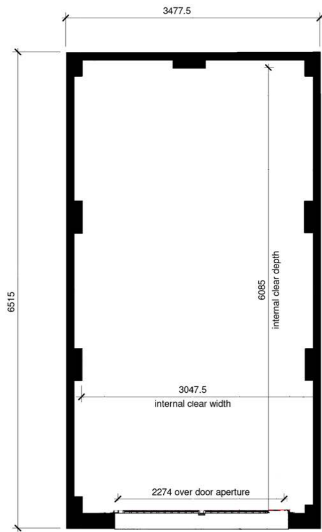
Floor Plan - Scale 1:50
